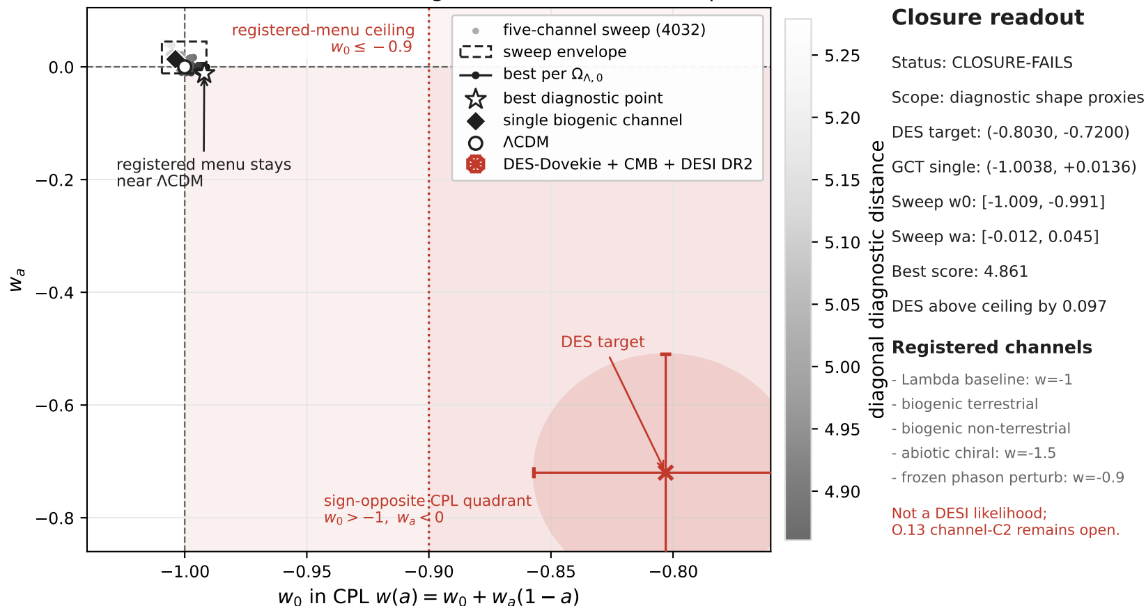
Figure V2.14.3. The DES-Dovekie+CMB+DESI DR2 diagnostic target lies in the quintessence-today, more-phantom-into-past quadrant; the registered five-channel shape menu remains near \Lambda CDM and cannot reach the DES central w_0 above the -0.9 ceiling.
